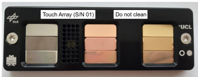
Figure 1. - Touch Array.
